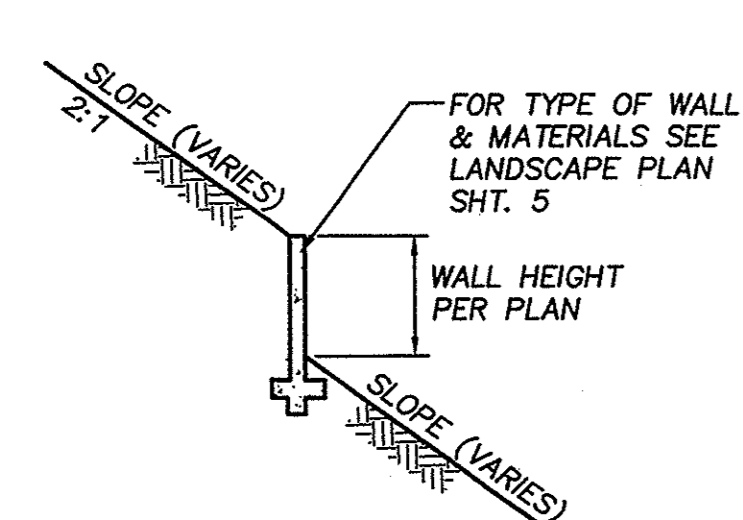
TYPICAL RETAINING WALL NOT TO SCALE
