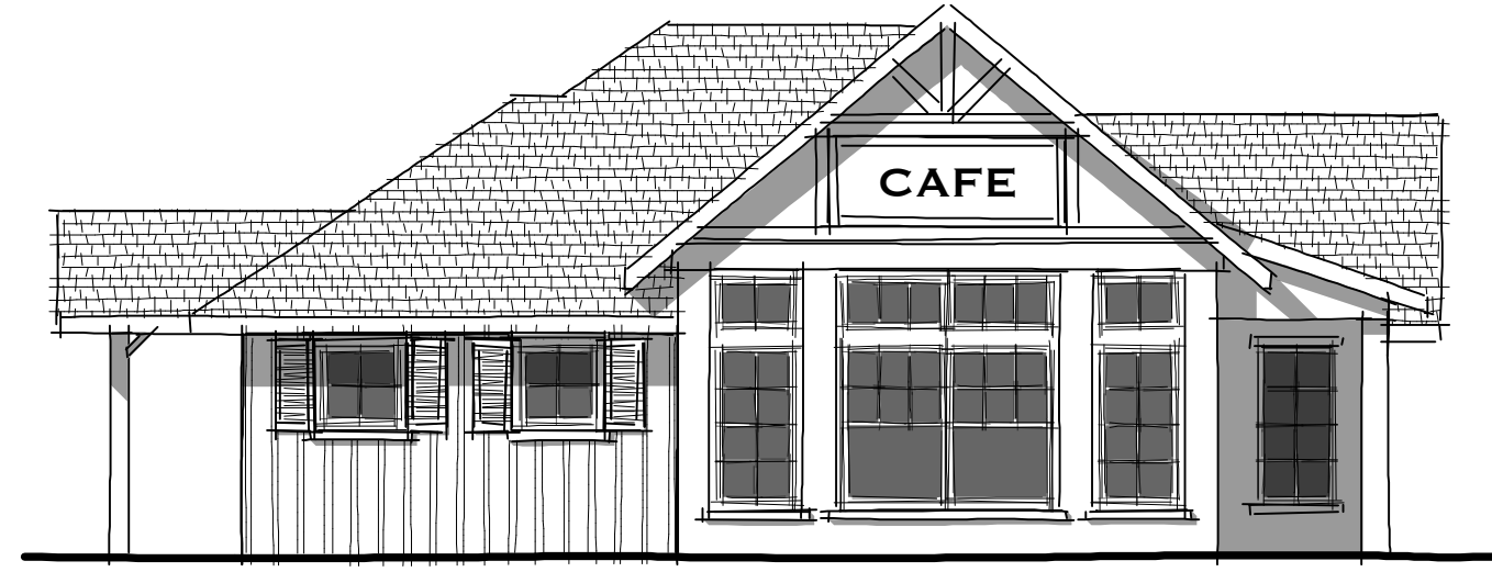
LEFT ELEVATION G - RANCHO SANTA FE ROAD VIEW
